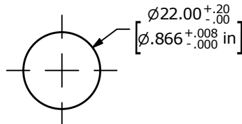
RECOMMENDED PANEL CUTOUT MAX. PANEL THICKNESS 10.0 [.39 in]
