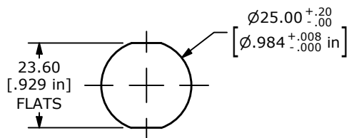
RECOMMENDED PANEL CUTOUT MAX. PANEL THICKNESS 10mm
