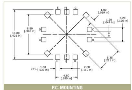
P.C. MOUNTING
