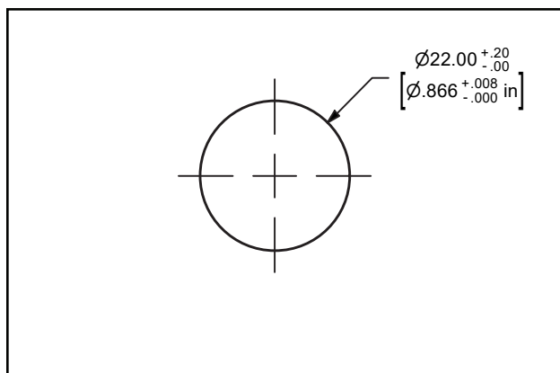
PANEL CUTOUT
